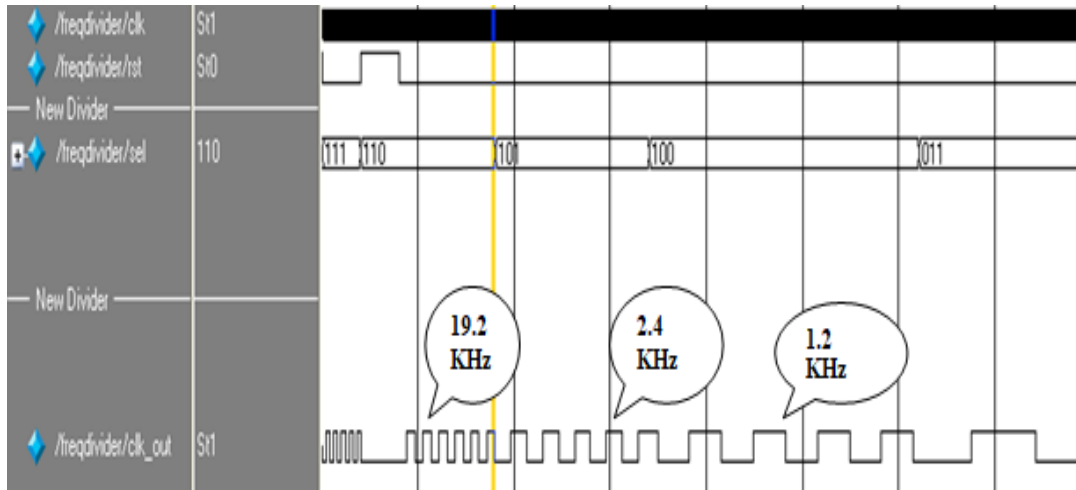
Figure 9. Simulation results of variable clock frequencies in proposed 16-QAM transceiver
