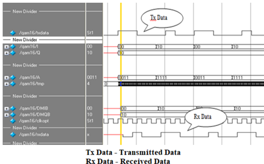
Figure 12 Simulation results of transmitted and received bit patterns
