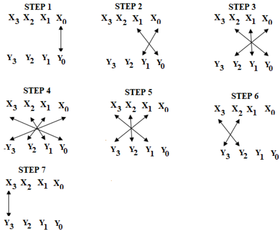
Figure 2 Urdhva Tiryakbhyam multiplication of two 4-bit binary number
