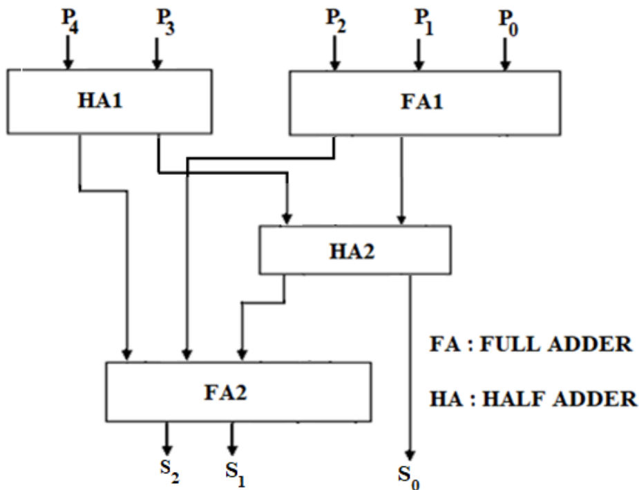
Figure 3. 5-3 compressor adder with half adders and full adders
