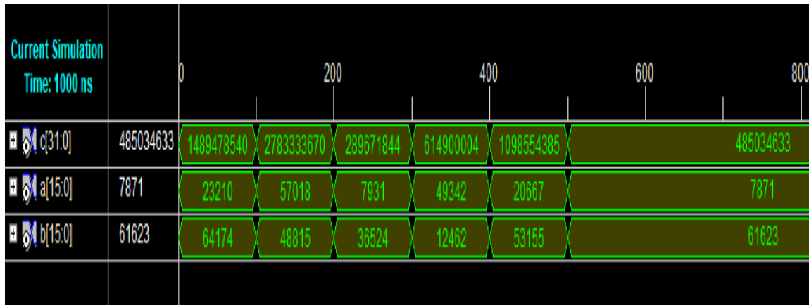
Figure 11 Functional simulation of 16-bit Vedic multiplier
