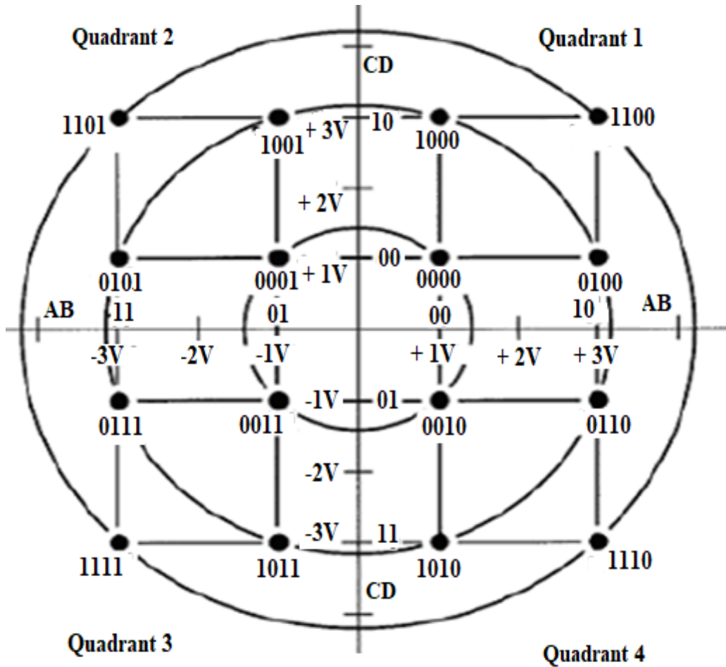
Figure 1 Constellation diagram of 16-QAM
