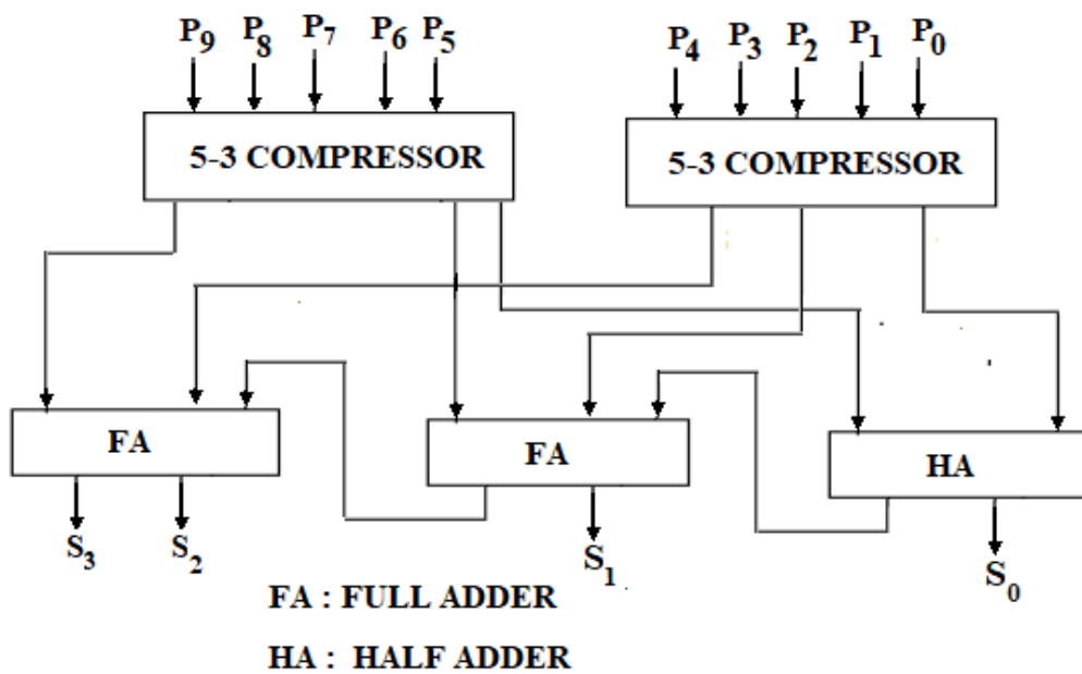
Figure 4. 10-4 compressor adder using 5-3 compressor adders
