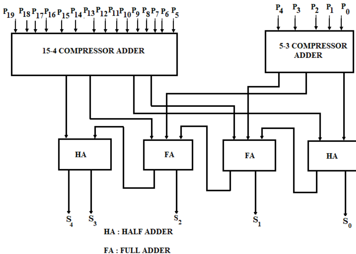
Figure 5 20-5 compressor adder using 15-4 and 5-3 compressor adder
