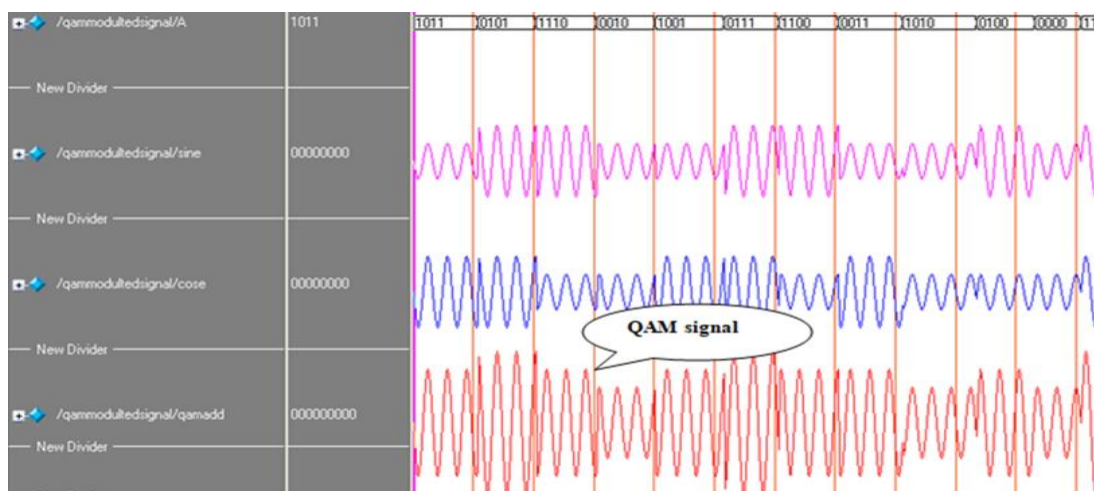
Figure 10 Simulation waveforms of QAM signal
