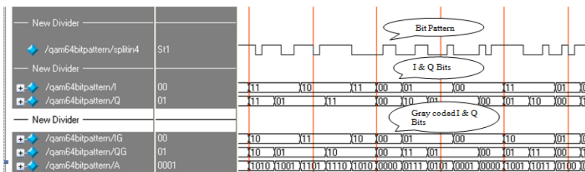
Figure 8 Simulation results of proposed 16-QAM transmitter
