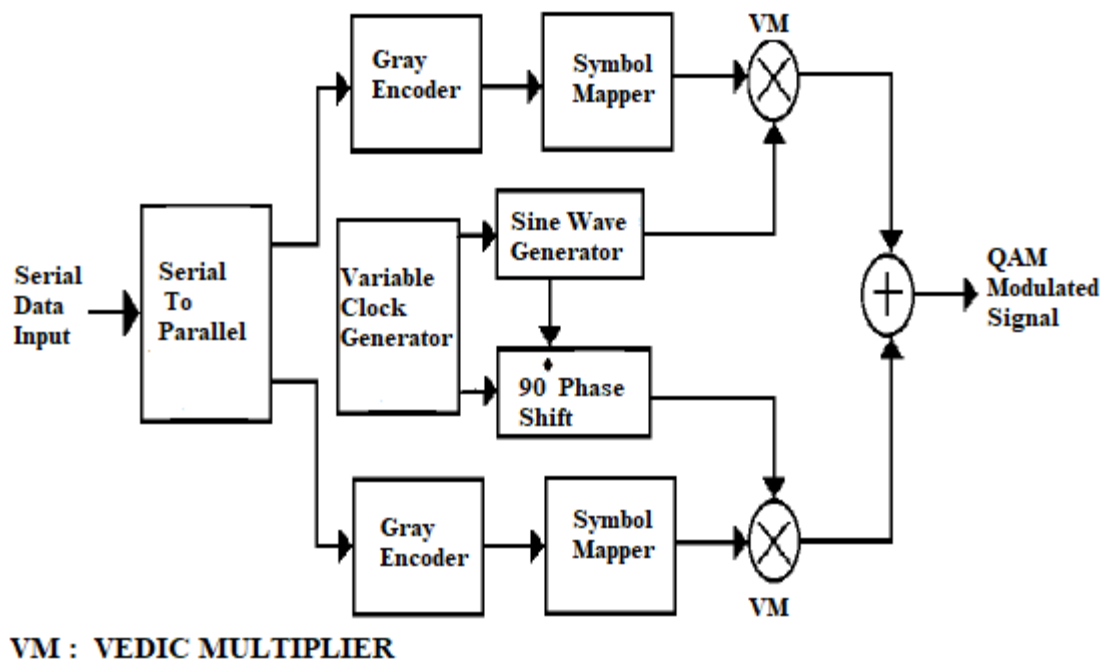
Figure 6 Block diagram of proposed QAM transmitter
